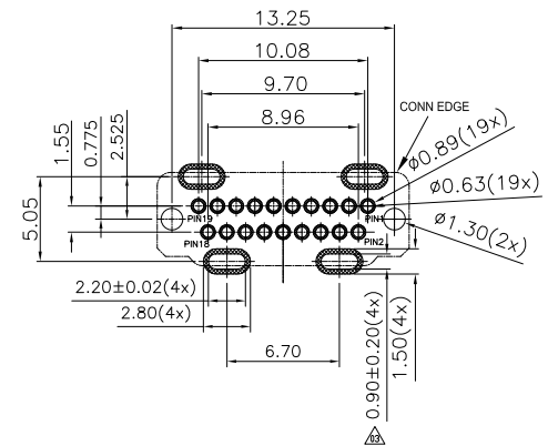
RECOMMENDED PCB LAYOUT (TOP VIEW) GENERAL TOLERANCES: ±0.05 (t=1.6/1.2)
