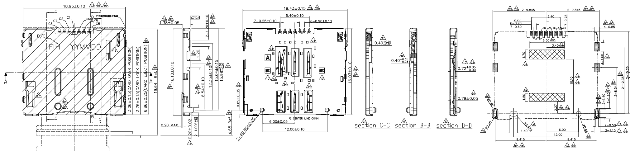
RECOMMENDED P.C.B LAYOUT(TOP VIEW) (General Tolerance±0.05)
