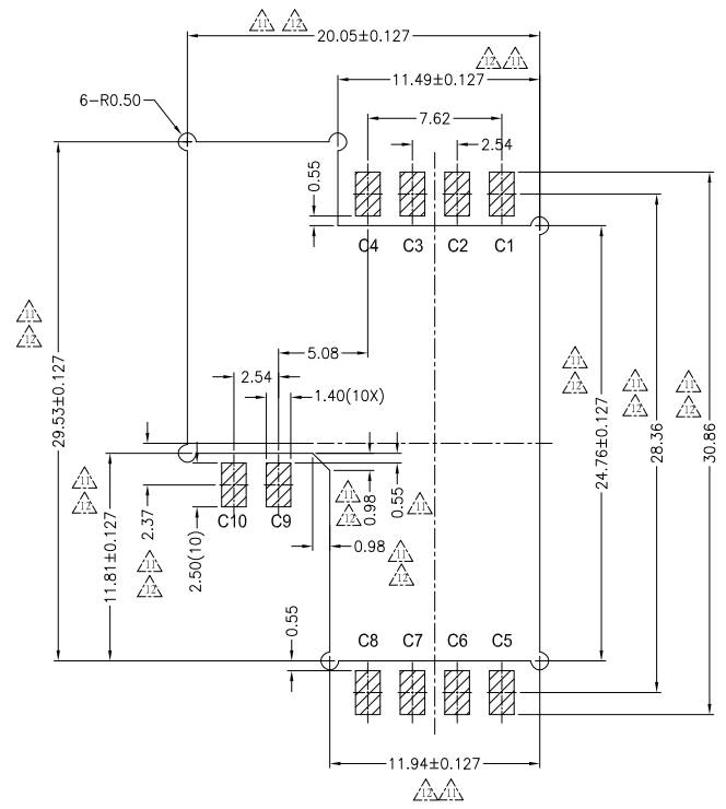
RECOMMENDED PCB LAYOUT (TOP VIEW) GENERAL TOLERANCES: ±0.05 (t=0.6)
