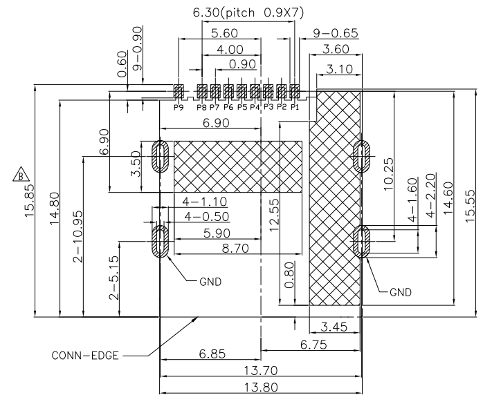
PCB PATTERN LAYOUT (GENERAL TOLERANCE:±0.05)
