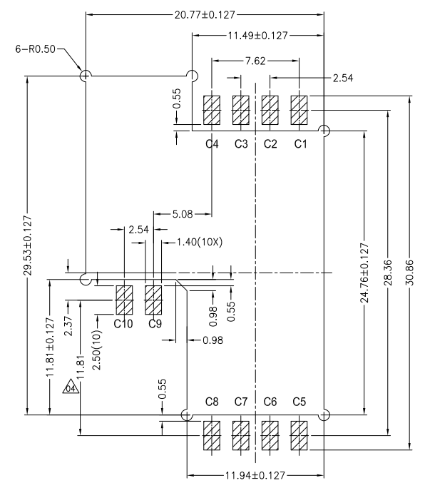
RECOMMENDED PCB LAYOUT (TOP VIEW) GENERAL TOLERANCES: ±0.05 (t=0.6)
