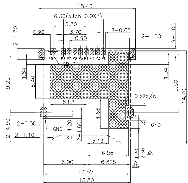
PCB PATTERN LAYOUT (GENERAL TOLERANCE:±0.05)
