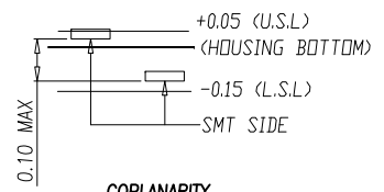
COPLANARITY
